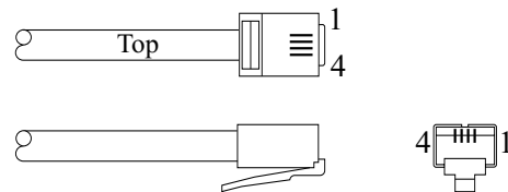
Conventional Pin Configuration Handset Plug
