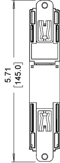
Rear View
