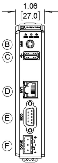
Top View
