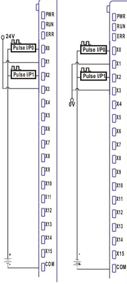
2. Single Phase Up counter
