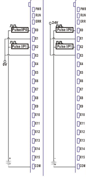
3. Single Phase Down counter
