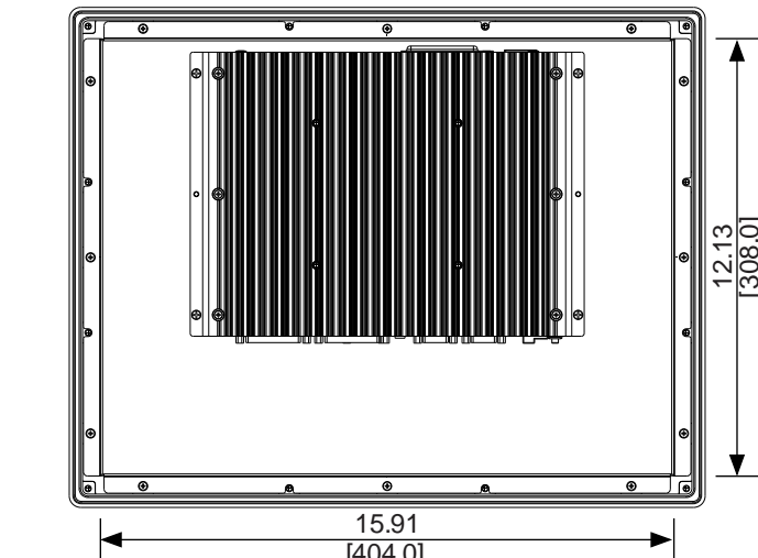
Rear View
